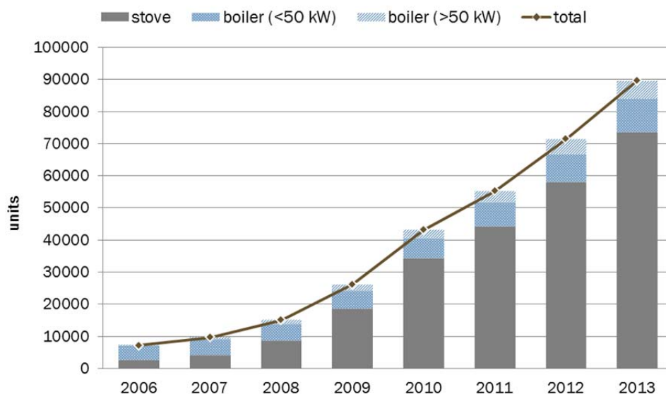
Figure 3.80 - Development of installed pellet heating systems in Spain from 2006 to 2013 (AEBIOM, 2013, 2012; AEBIOM's National Biomass Boiler Observatory, 2011)
