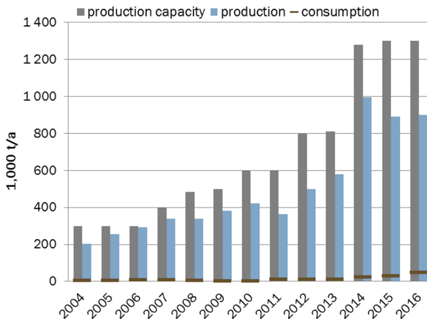
Figure 3.7 - Wood pellet market development in Estonia from 2004 to 2016.
