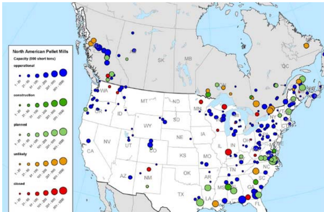
Figure 4.10. - Geographic location of North American Pellet Mills (Source: http://i.bnet.com/blogs/north-american-pellet-mills.jpg )
