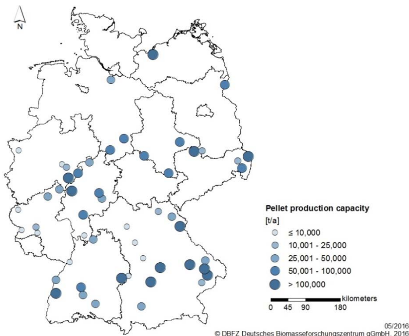
Figure 3.40 - Location of wood pellet production plants in Germany 2015 (this overview makes no claim of being complete) (Berner, 2015).
