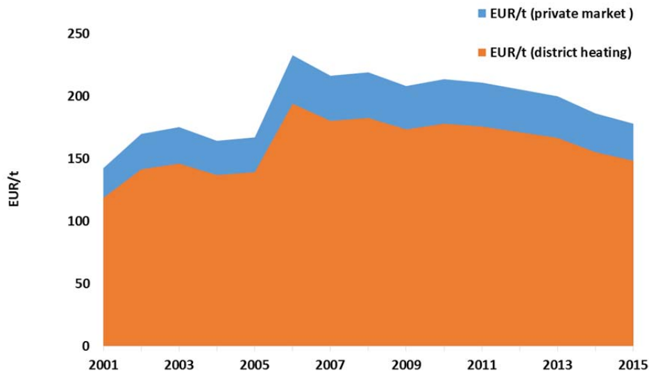
Figure 3.24 - Price development for wood pellets delivered in bulk to private consumers and district heating utilities. Graph is based on data from Danish District Heating organization, Danish Energy Agency and by personal communication with end-users and pellet providers.
