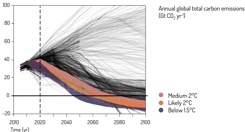
Source: Rogelj et al., 2015, Nature Climate Change. Based on 200 Message and Remind scenarios
