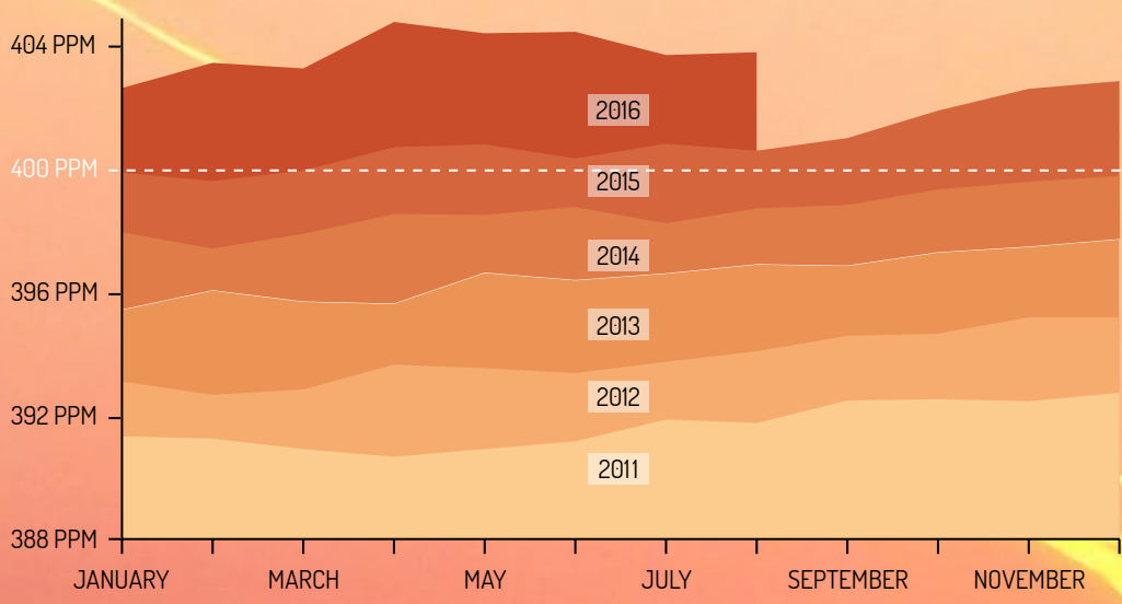
Source: Scripps Institute of Oceanography Mauna Loa Observatory
